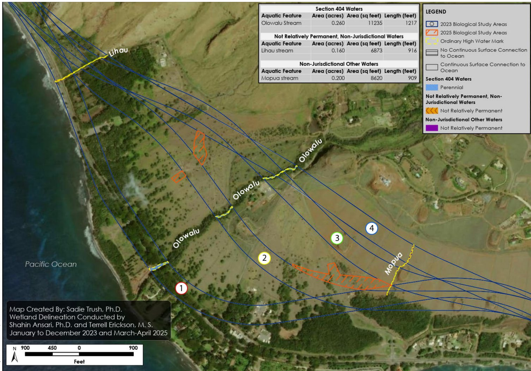
FIGURE 3.9-3. Preliminary Other Waters of the U.S. Delineation – Olowalu
