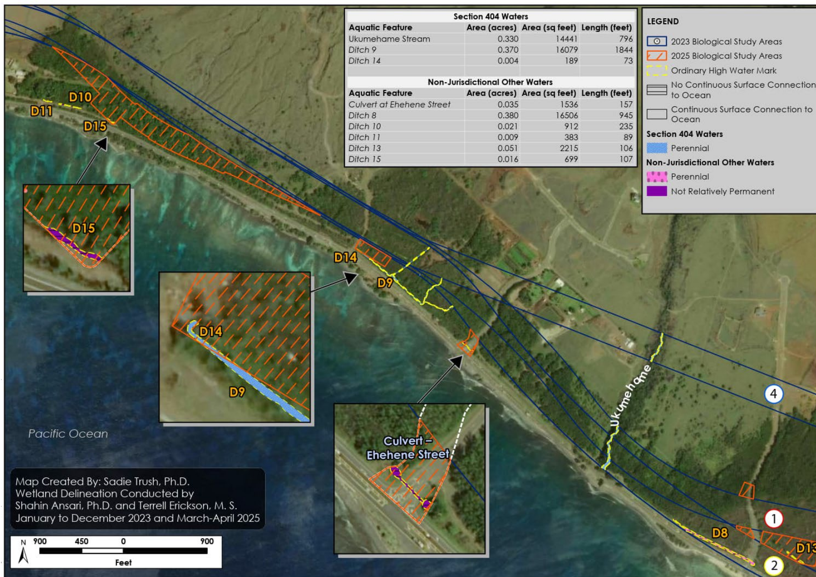
FIGURE 3.9-2. Preliminary Other Waters of the U.S. Delineation – Common Alignment and Ukumehame Area
